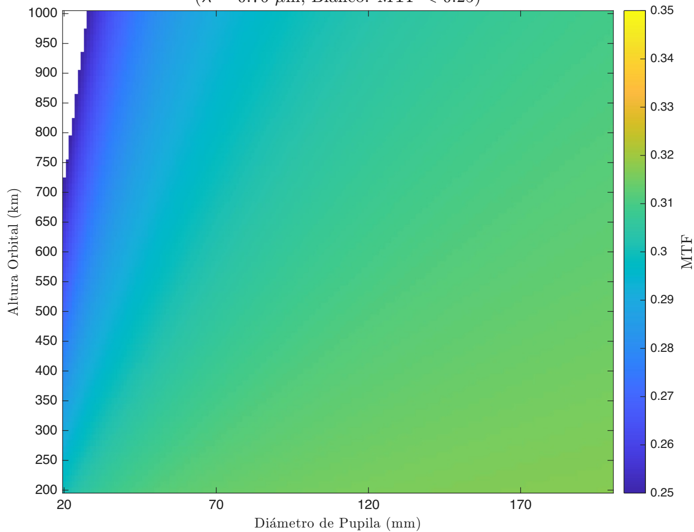
MTF - Refractivo - Detector 3 ( \lambda = 0.76 \mu\text{m} , Blanco: MTF < 0.25)
